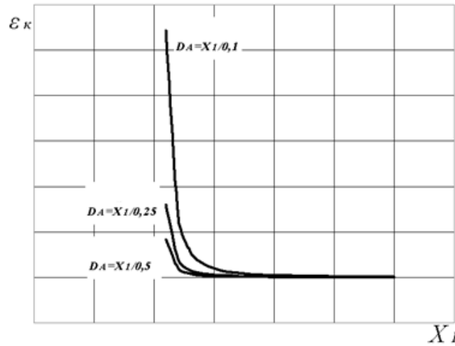
Figure 4: Graphs of coefficient for resistant ek cone valve moving at different ratios X_1 and outside diameter D_A channel
