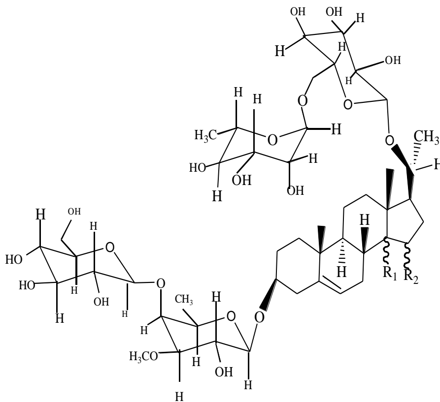
Fig 1: lasianthoside-A and lasianthoside-B Lasianthoside-A -R 1 , R 2 = \Delta^{14-15} , Lasianthoside-B -R 1 = \beta -OH, R 2 = H R 1 = \beta -OH, R 2 = H
