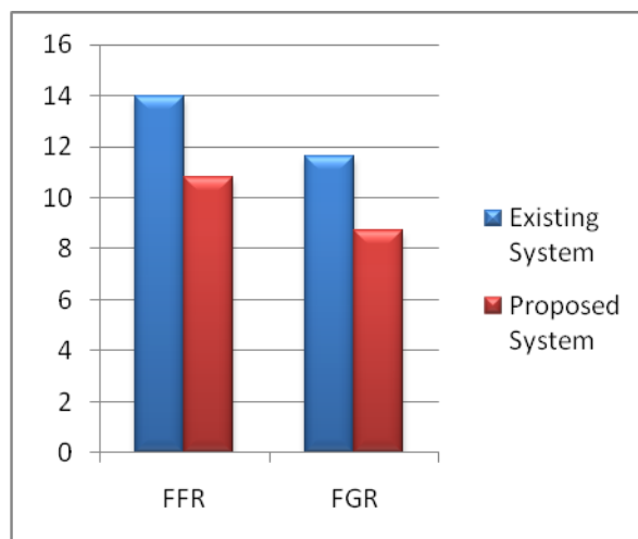
Figure 6. Performance evaluation
