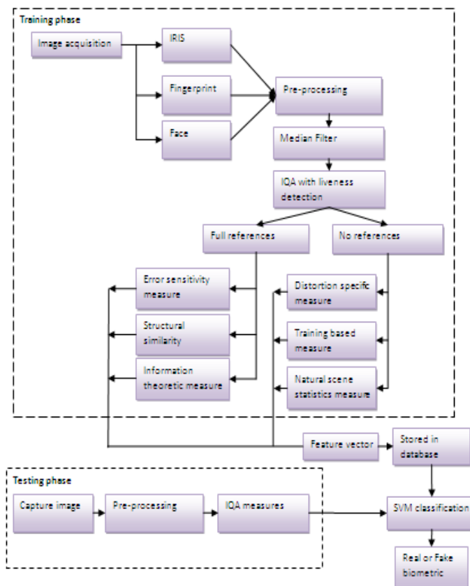
Figure 2. Proposed Framework
