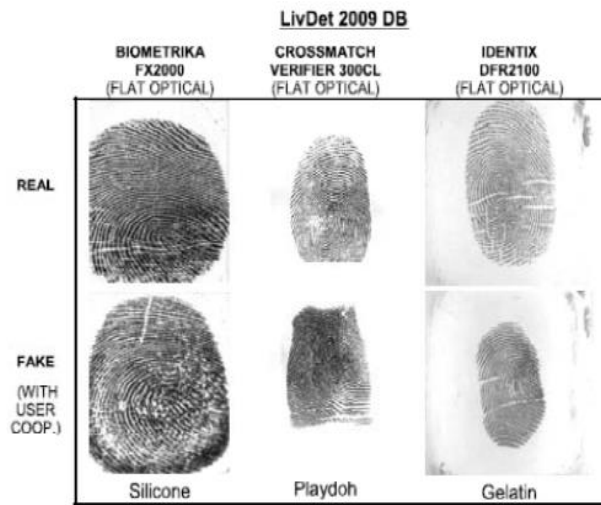
Figure 3. Fingerprint datasets
