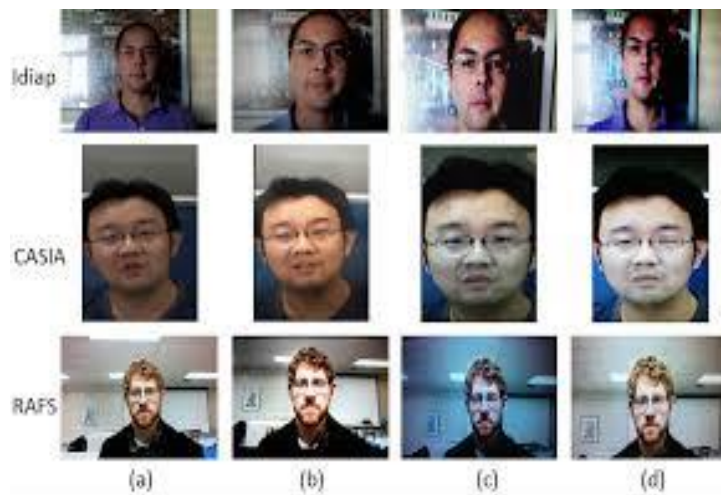
Figure 5. Face datasets
