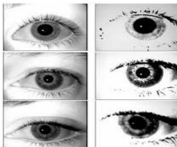
Figure 4. IRIS datasets
