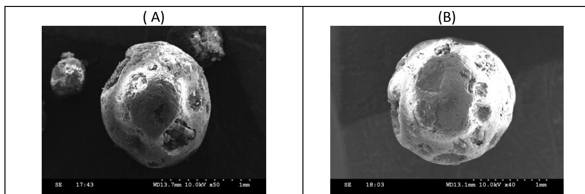
Fig.1. SEM of Olibanum Resin Coated Microcapsules of Aceclofenac F2 Prepared Employing Chloroform (A) and Microcapsules F6 Prepared Employing Dichloromethane (B) as Solvents for the Polymer
