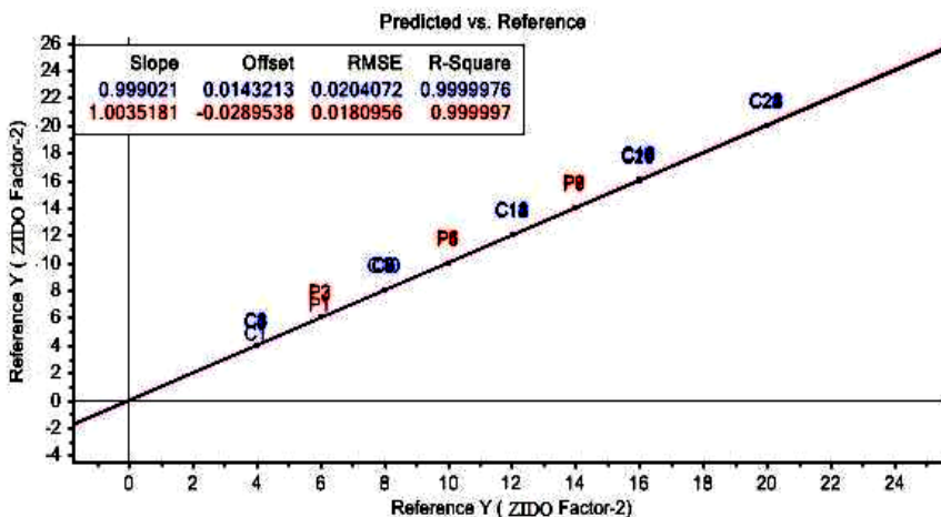
Graph 2: Calibration and prediction spectra of Zidovudine
